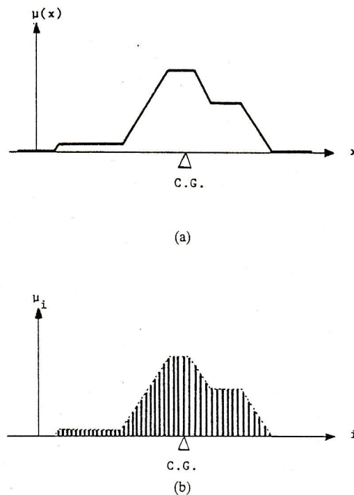
Fig. 6. Defuzzification (center-of-gravity method) of (a) a continuous membership function and (b) a discrete membership function.
