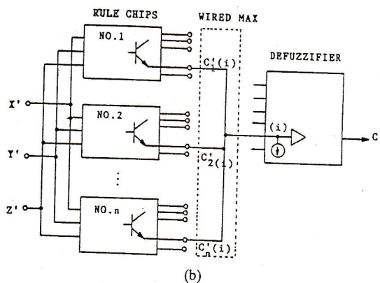
Fig. 16. (a) Aggregation of individual conclusions (individual inference results) with a MAX array. (b) Aggregation by wired MAX.
