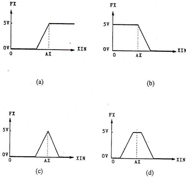
Fig. 11. Four types of membership functions realized by an MFC shown in Fig. 10. (a) S-function, (b) Z-function, (c) \Delta -function (triangular function), and (d) \Pi -function (trapezoidal function).
