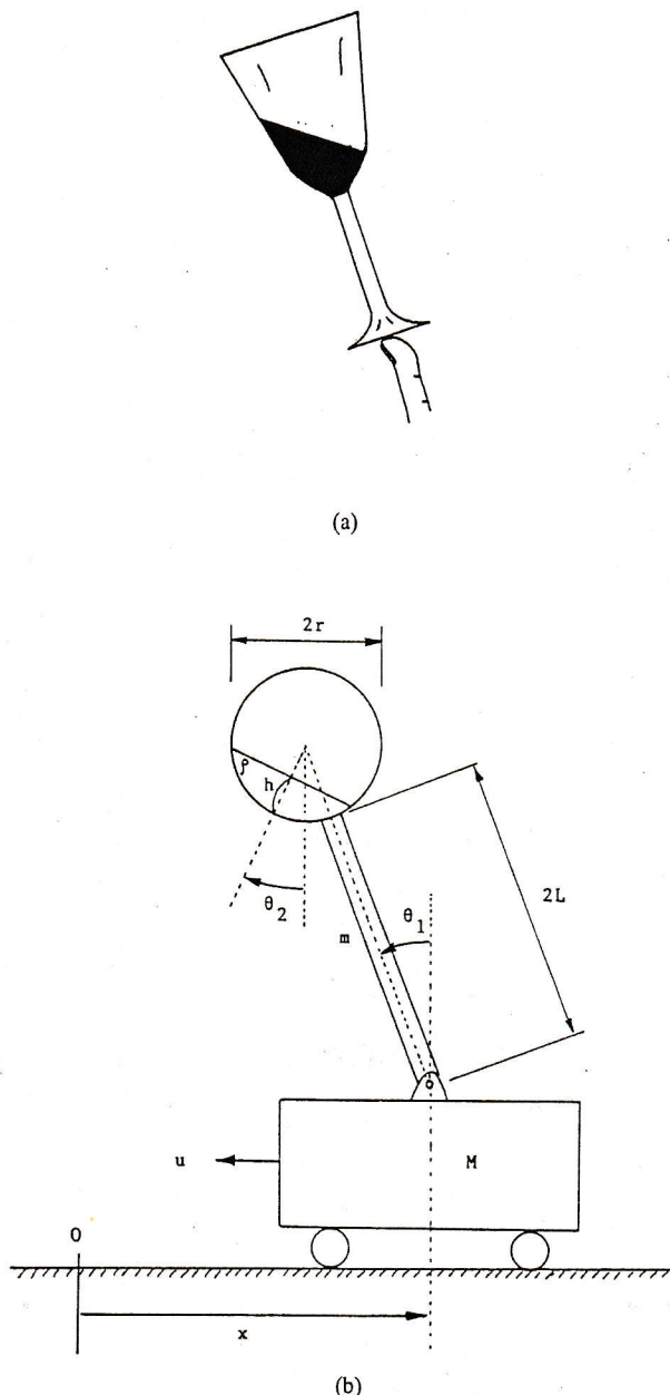
Fig. 28. (a) Stabilization of a glass with wine on a finger tip. (b) A simplified model of the glass stabilization.
