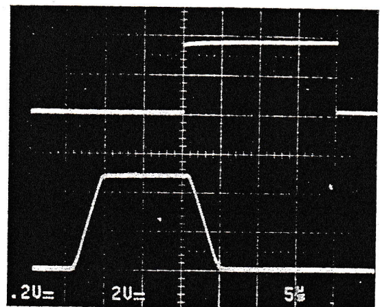
Fig. 20. A step response of the defuzzifier.
