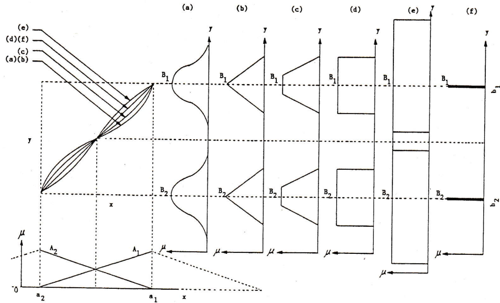
Fig. 21. Comparison of interpolation between some fuzzy inferences.
