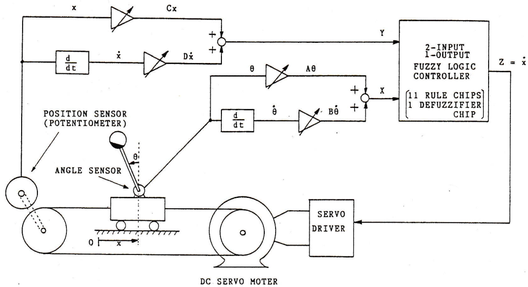
Fig. 30. A block diagram of a wine glass stabilization.
