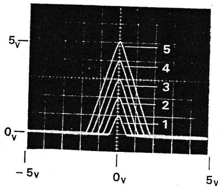
Fig. 22. A grade-controllable membership function circuit (GC-MFC). It is obtained by modifying the ordinary membership function circuit.
