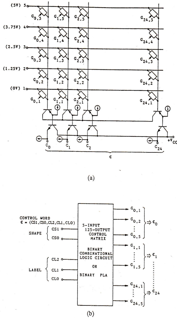
Fig. 14. Main blocks of a membership function generator. (a) A switch matrix and an emitter follower array (b) a control matrix.
