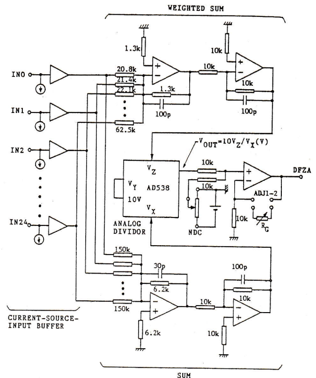
Fig. 19. A circuit configuration of the defuzzifier.
