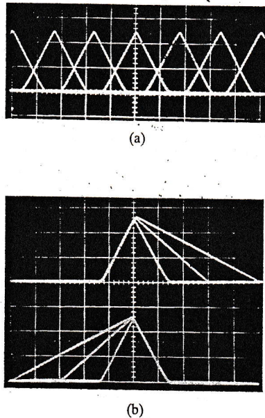
Fig. 12. Input-output characteristics of a membership function circuit (MFC). (a) \Delta -functions for various labels ( AX = -5 V, -3.3 V, -1.7 V, 0 V, 1.7 V, 3.3 V, 5 V). (b) \Delta -functions for various slopes. (Upper: R_{XR} = 120 \Omega, 266 \Omega, 444 \Omega, R_{XL} = 120 \Omega . Lower: R_{XL} = 120 \Omega, 266 \Omega, 444 \Omega, R_{XR} = 120 \Omega ).
