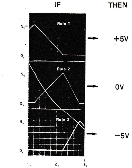
Fig. 26. Membership functions of NL (top), PS (middle), and PL (bottom) which are used in the antecedents of three rules for testing a singleton controller.
